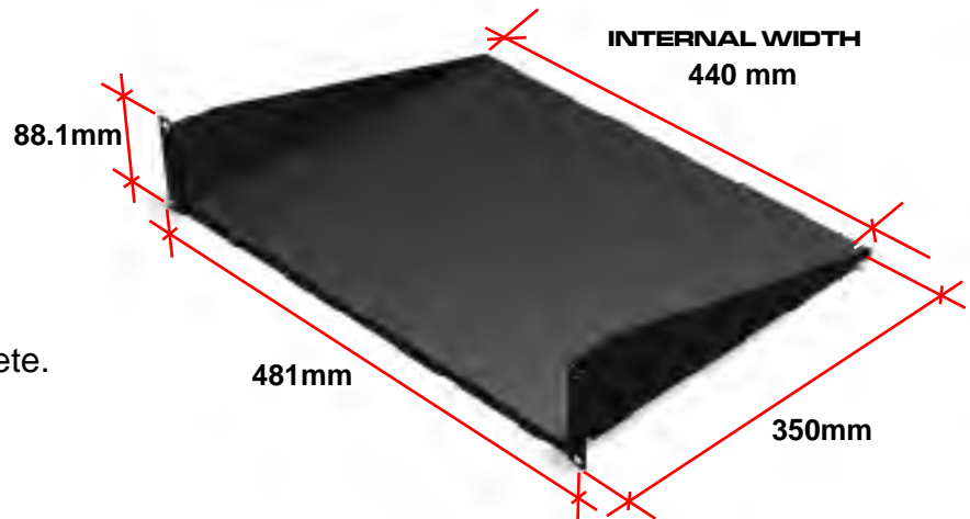
OVERALL DIMENSIONS
